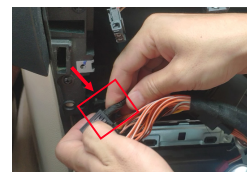
11. Insert the fiber cable into iSmart auto box 48PIN harness
