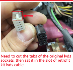
8. Connect CarPlay's LVDS cable with the original car's video
